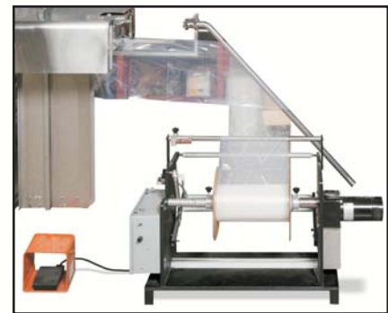
Controlled tension with driven unwind stand to handle large diameter rolls for longer production runs.
